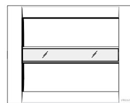
Classica cover plate 16748... Technopolymer, with signalling tags Available colours: bright white (01), Idea white (04), Idea grey (14), black (16), metallized anthracite (V23). Dimensions: 206x150x11 mm
