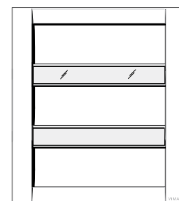
Classica cover plate 16749... Technopolymer, with signalling tags Available colours: bright white (01), Idea white (04), Idea grey (14), black (16), metallized anthracite (V23). Dimensions: 206x222x11 mm
